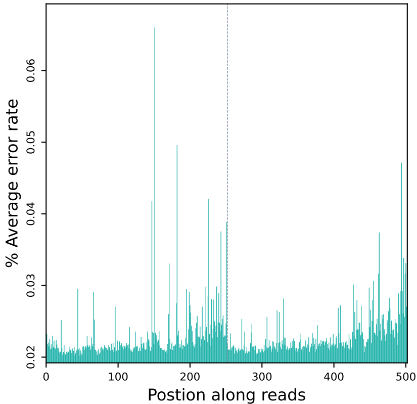
Error rate distribution along reads (R10427)
